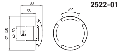
Accessorio controcassa cod 101500 Outer casing accessory, code 101500
